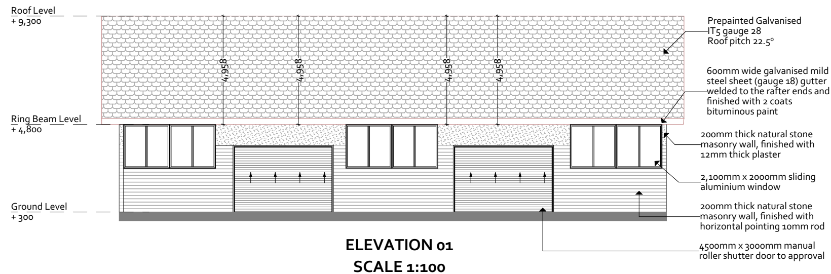
ELEVATION 01 SCALE 1:100
