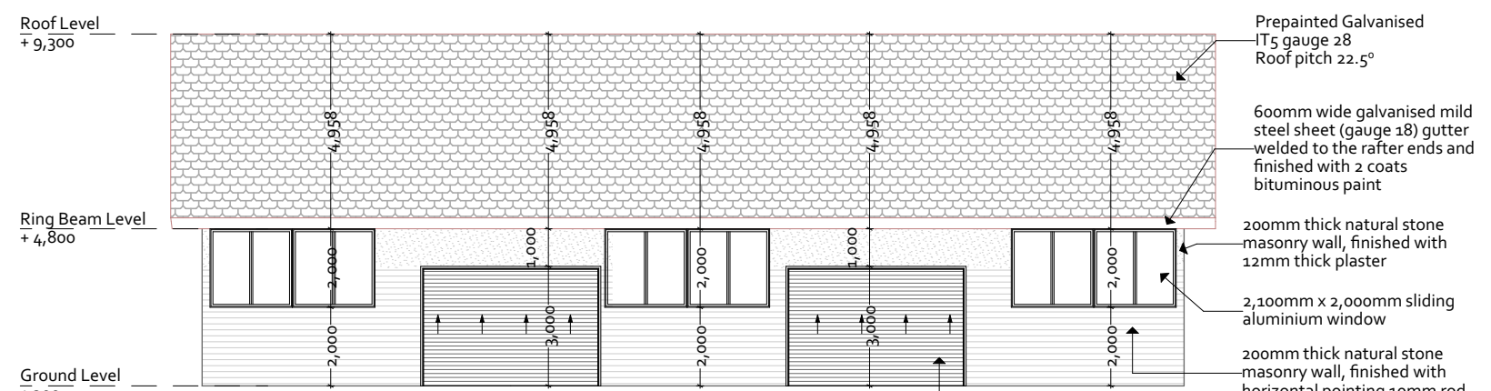
ELEVATION 03 SCALE 1:100
