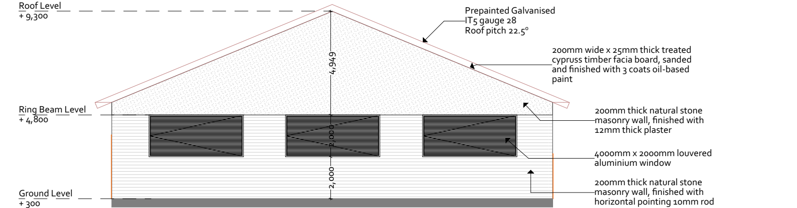
ELEVATION 02 SCALE 1:100
