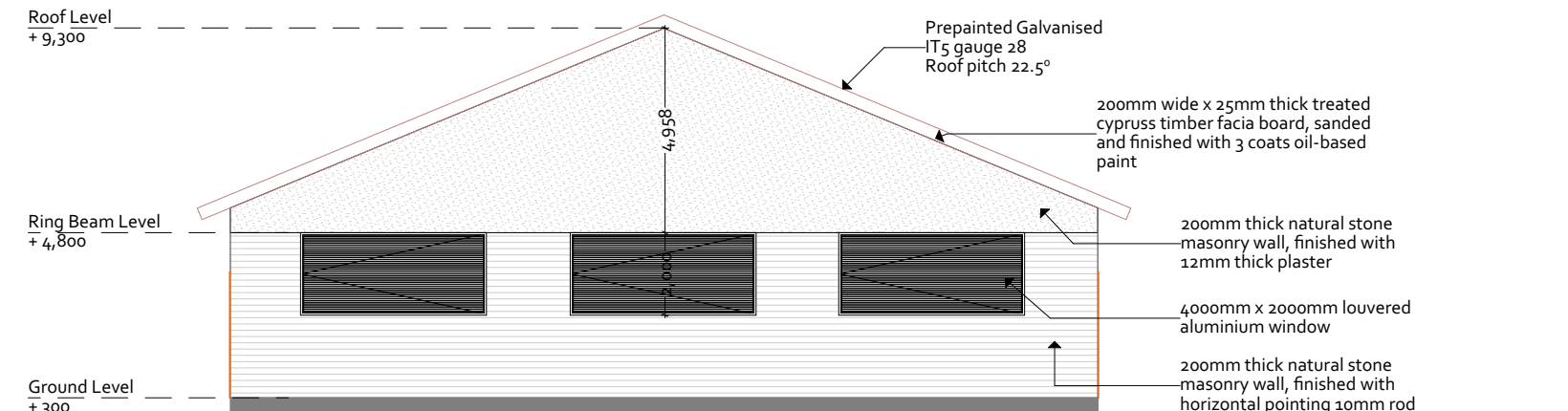
ELEVATION 04 SCALE 1:100
